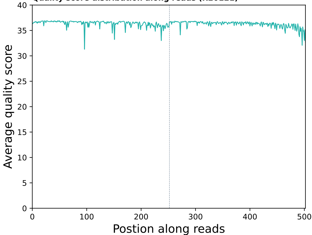
Quality score distribution along reads (R20121)
